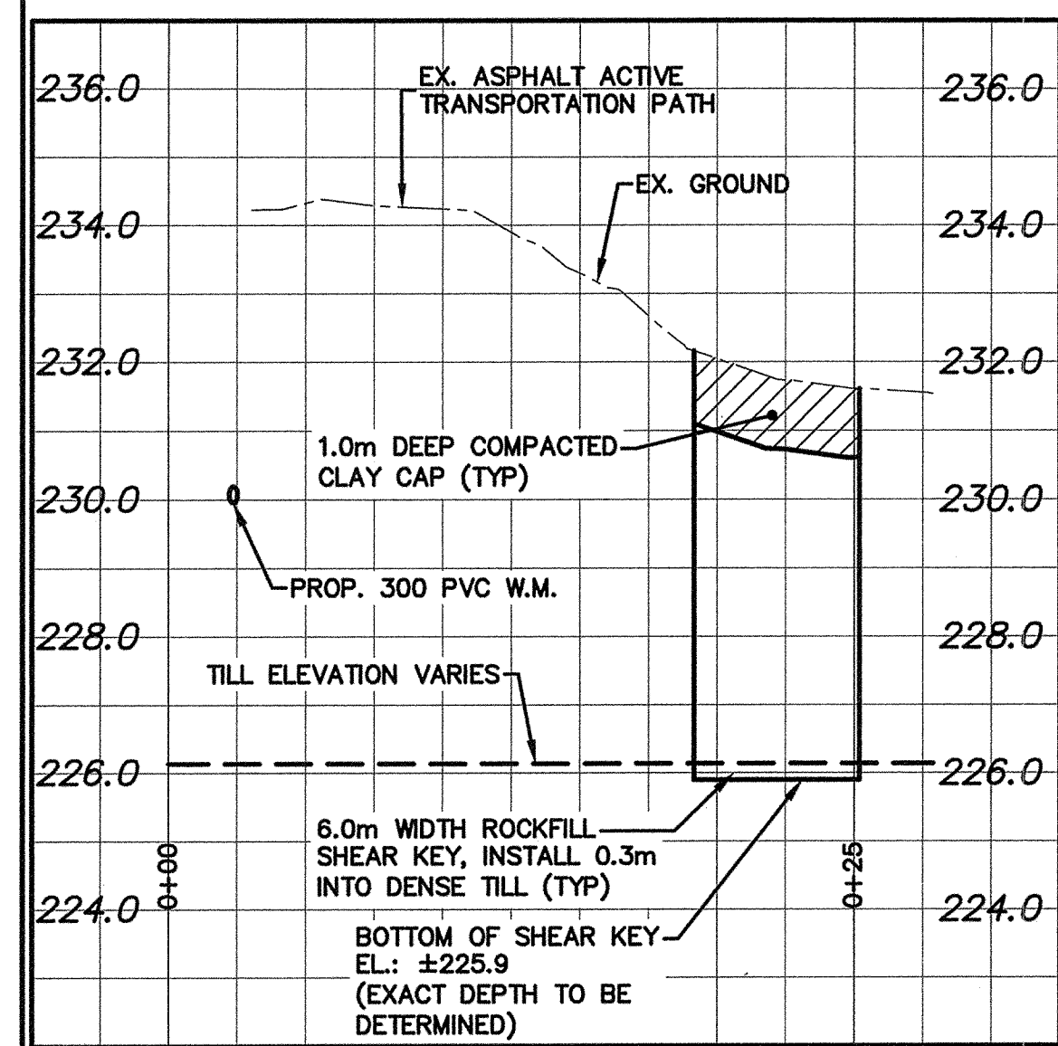
NORTH BANK CROSS SECTION SCALE: H=1:250, V=1:100
